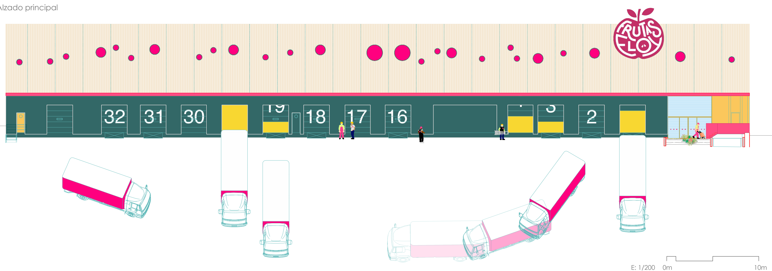
Alzado principal
